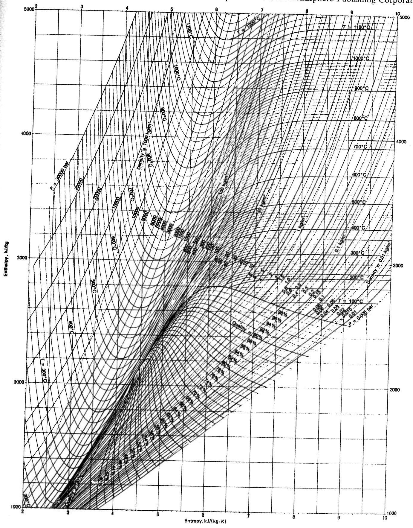
Mollier diagram for water. (Source: Lester Haar, John S. Gallagher, and George S. Kell, NBS/NRC Steam Tables . With permission from Hemisphere Publishing Corporation, 1972)
