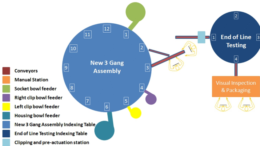
Fig. 10. Proposed layout for Cell 2 (Concept 1)
