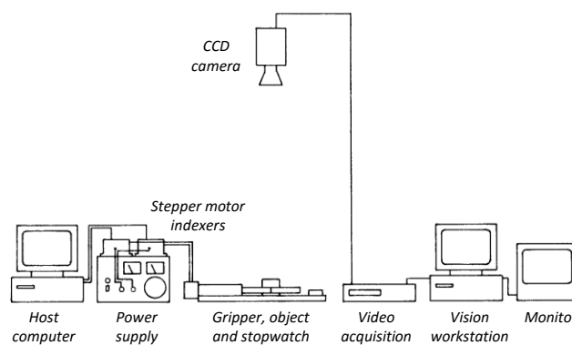
Fig. 8. Experimental set-up.
