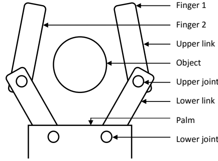
Fig. 1. Basic configuration of an underactuated hand.
