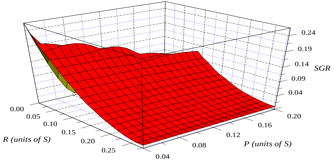
Fig. 18. Variation of peak SGR with P and R at L_r = 0.75
