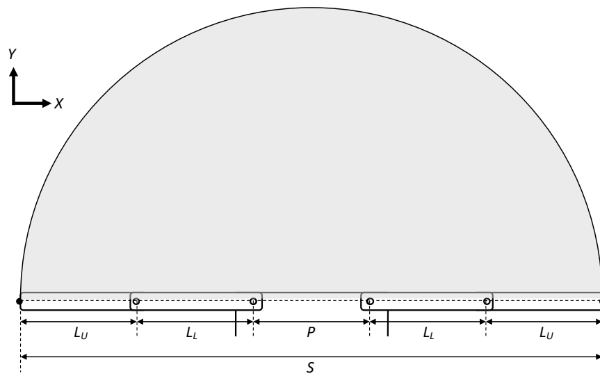
Fig. 10. Workspace of the robot gripper.
