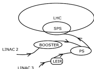
Figure 3 – Schematic diagram of CERN accelerators
