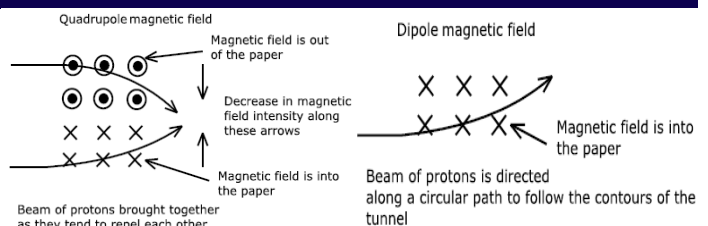
Diagram 4 — Quadrupole magnetic field to focus beam Figure 5 – Dipole magnetic field to direct beam
