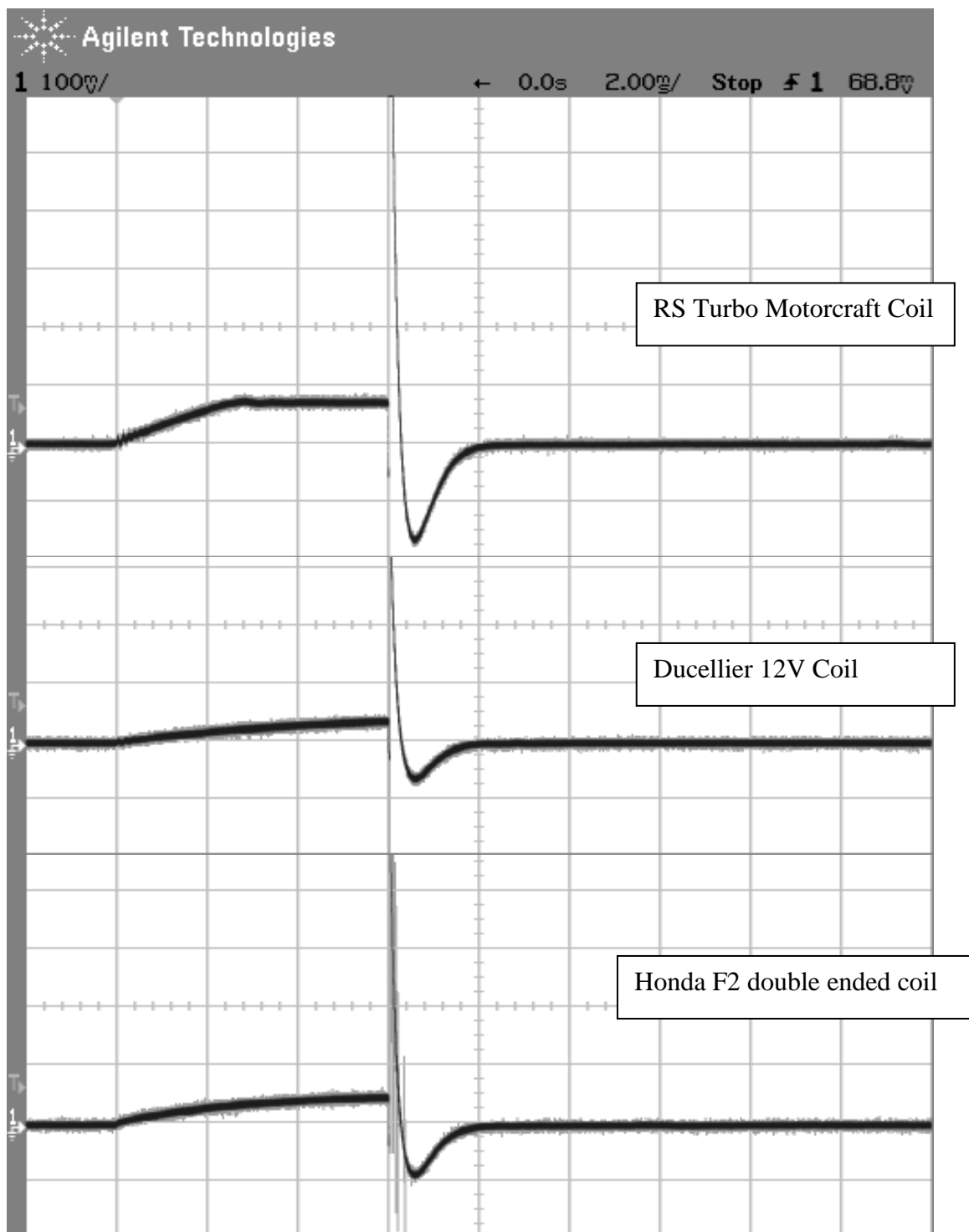
Figure 7 Current curves through various 12V ignition coils
