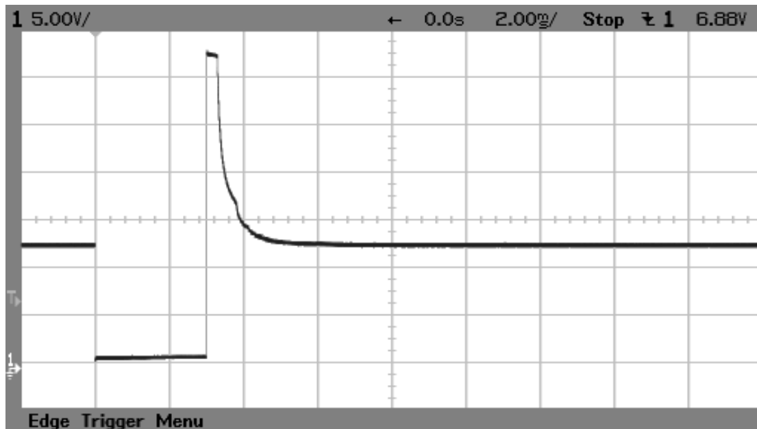
Figure 6 Current and voltage curves, high impedance injector 3ms DOI
