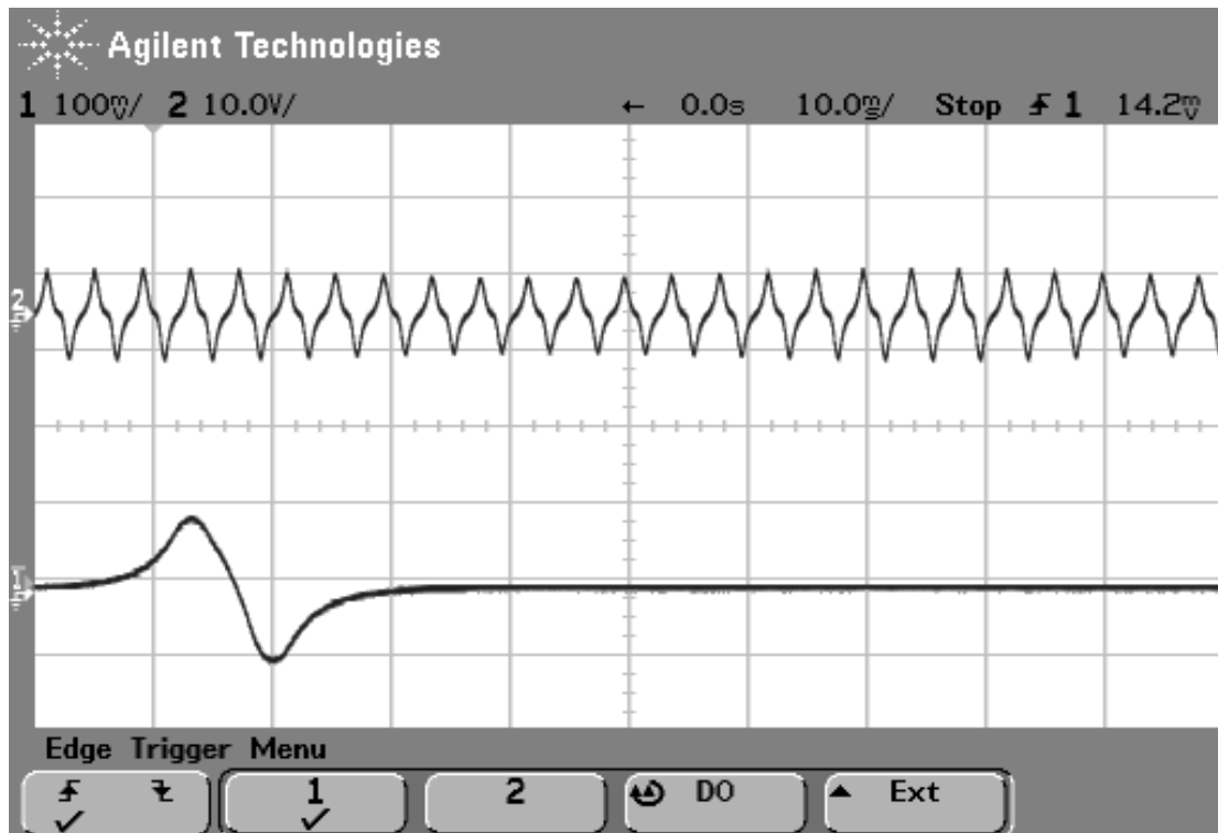
Figure 3 Signals from Cam and Crank sensors
