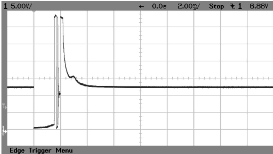
Figure 5 Current and voltage curves, DOI 2ms, low impedance injector
